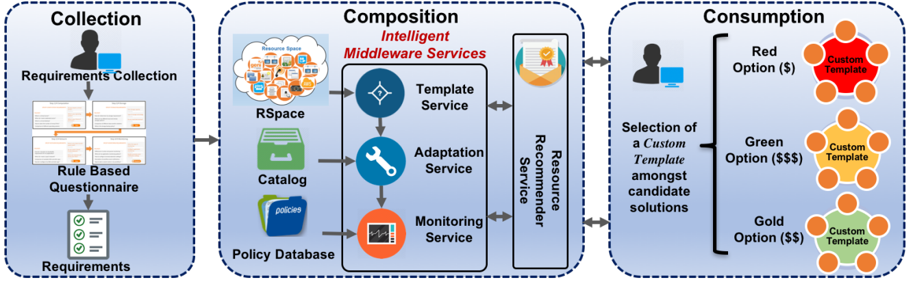
Figure 2: Custom Template Life Cycle. Our middleware solution presents three main stages: (a) Collection, that abstracts data-intensive application requirements. (b) Composition, that recommends template solutions based on the comparison of requirements with templates stored in a catalog or by the creation of new templates, and (c) Consumption, that enables cloud resource deployment automation.
